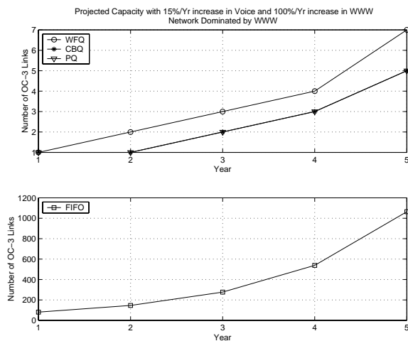
Figure 6.14: Network Capacity with Projections on Voice and WWWW Traffic
