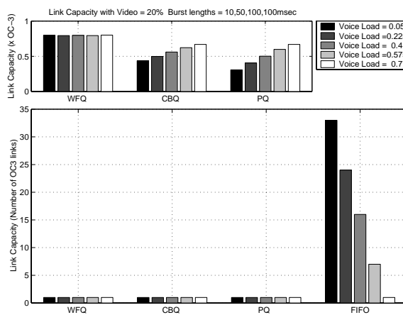
Figure 6.18: Link Capacity with varying burst sizes
