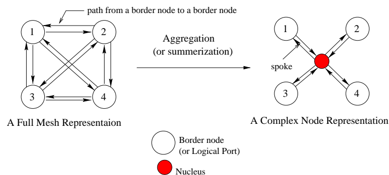
Figure 4.6: Nodal Aggregation
