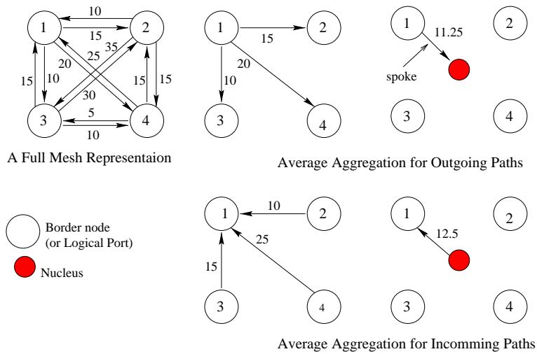
Figure 4.9: Average Aggregation Policy
