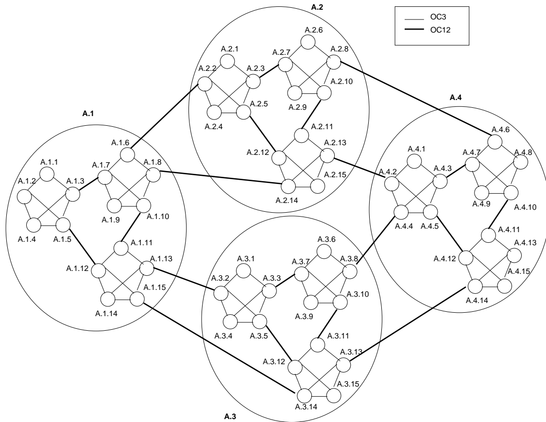
Figure 5.3: 4-Cluster Topology
