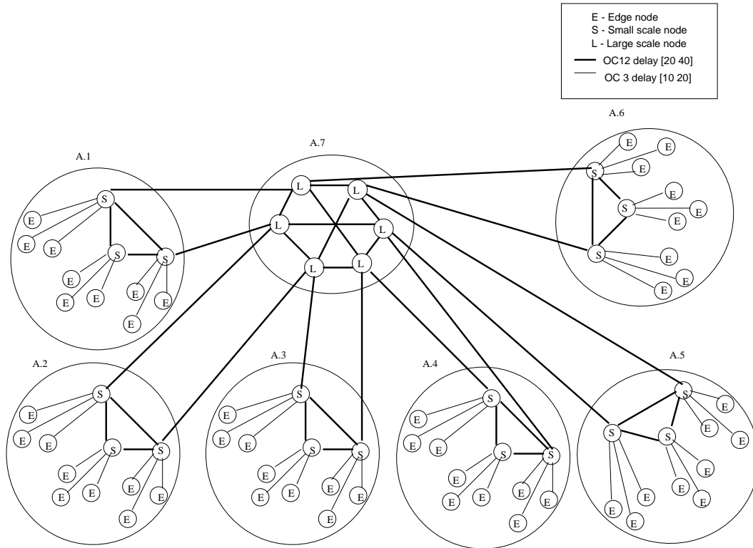
Figure 5.1: Edge-Core Topology
