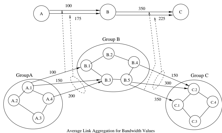
Figure 4.5: The Average Link Aggregation for Bandwidth Values
